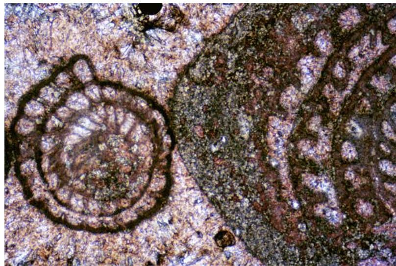
亮晶生物(纺锤虫)碎屑石灰岩
